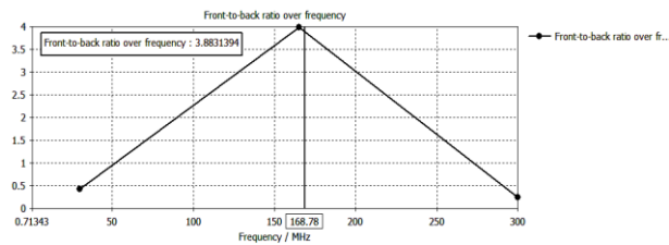
Figure 6: Front to back ratio of 4 element Yagi Uda antenna
