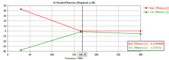
Figure 5: Efficiency of 4 element Yagi Uda antenna
