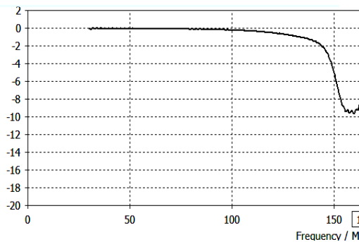
Figure 2: Return loss of 4 element Yagi Uda antenna
