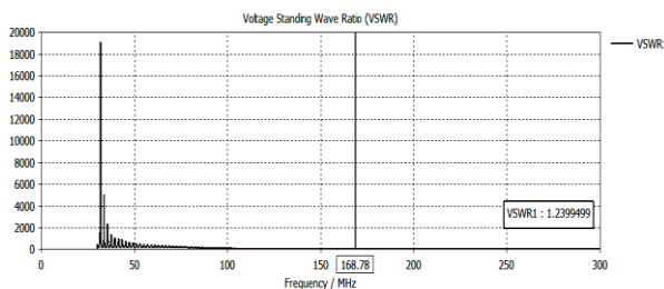
Figure 3: VSWR of 4 element Yagi Uda antenna
