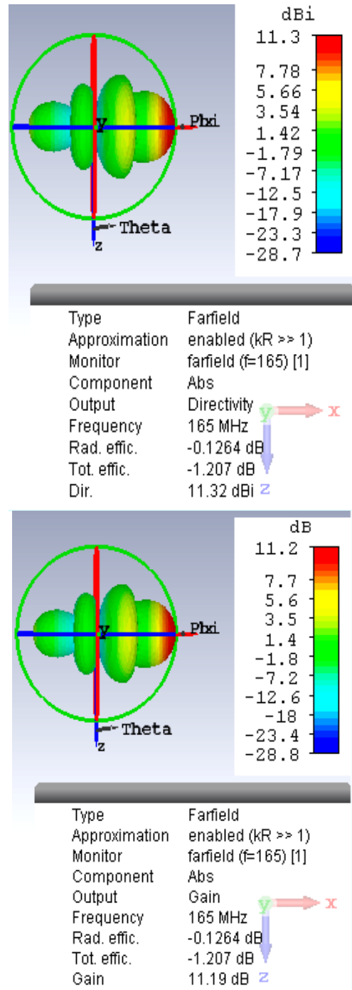
Figure 4: Directivity and Gain of 4 element Yagi Uda antenna
